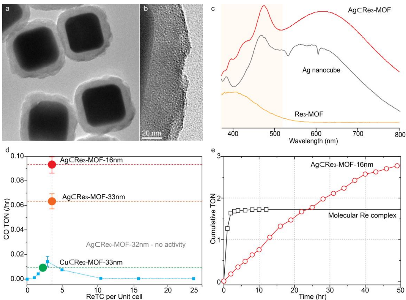
Figure 4. Characterization of Ag C Re 3 -MOF. (a) TEM image of Ag C Re 3 -MOF showing Re 3 -MOF constructed on the surface of a Ag nanocube. (b) Magnified image of Re 3 -MOF. (c) UV-Vis spectra of Re 3 -MOF, Ag nanocube, and Ag C Re 3 -MOF. (d) Photocatalytic CO 2 -to-CO conversion activity of Re n -MOFs, Ag C Re 0 -MOF, Cu C Re 2 -MOF, and Ag C Re 3 -MOFs with MOF thickness of 16 nm and 33 nm. (e) Stable performance of Ag C Re 3 -MOF compared to molecular H 2 ReTC.
