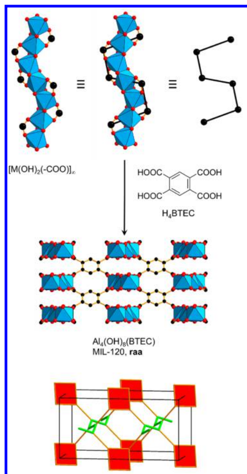
Figure 14. Single crystal structure of Al_4(OH)_8(BTEC) , MIL-120. The helical rod SBUs are connected by tetratopic organic linkers yielding a (3,4)-c raa net. 100 Color code: black, C; red, O; blue polyhedra, metal.
