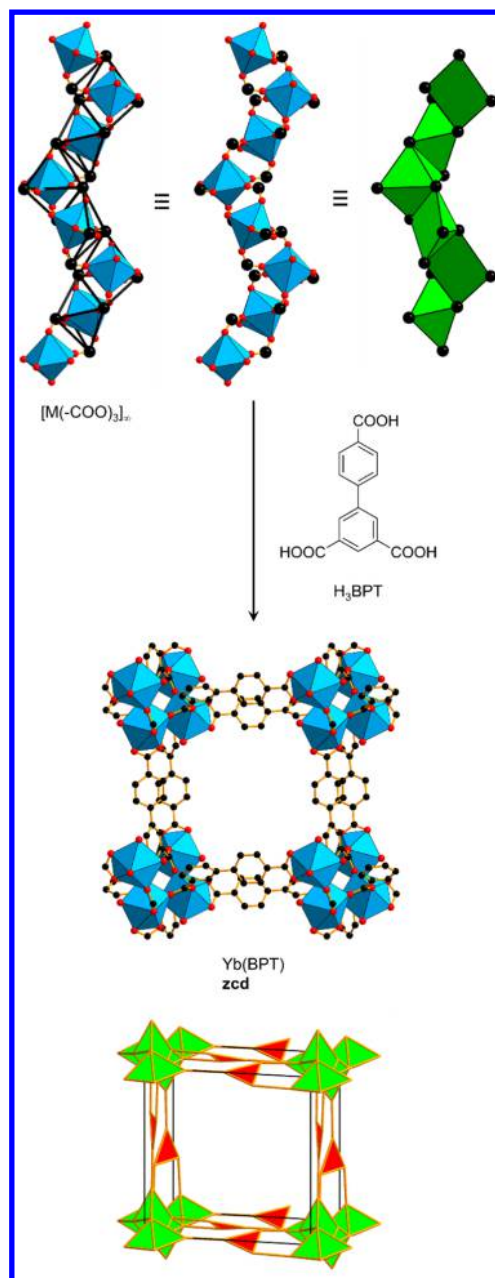
Figure 52. Combination of edge-sharing square pyramidal SBUs with tritopic BPT to produce \text{Yb}(\text{BPT}) showing a 6-nodal \text{zcd} topology. 211 Color code: black, C; red, O; blue polyhedra, metal.
