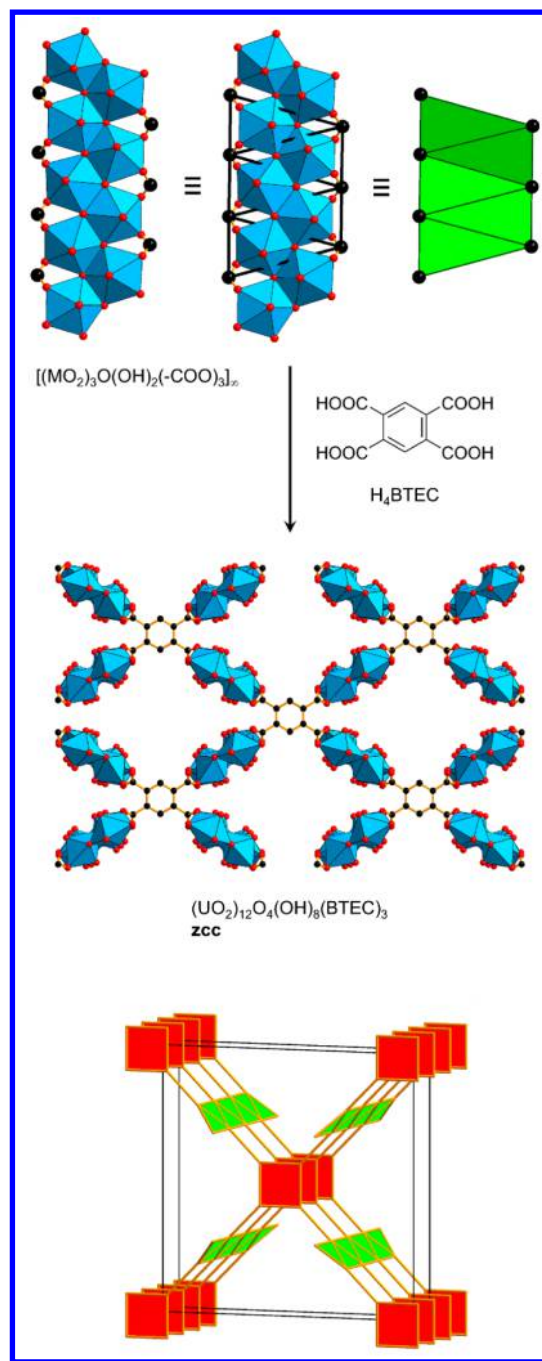
Figure 77. Crystal structure of (UO_2)_{12}O_4(OH)_8(BTEC)_3 . Rod SBU composed of edge-sharing triangles is linked with square nodes into a (3,4)-c zcc net. 241 Color code: black, C; red, O; blue polyhedra, metal.
