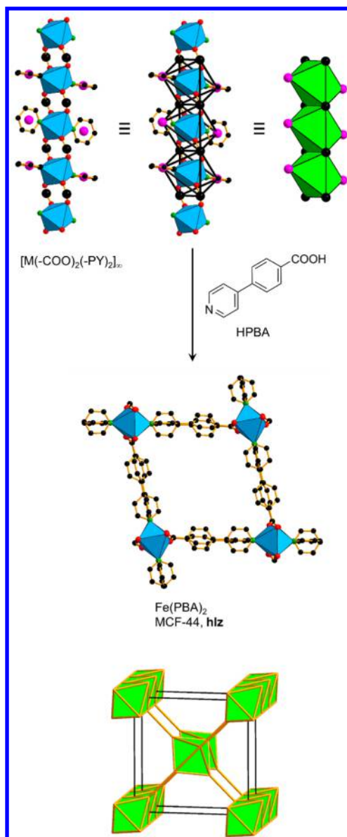
Figure 36. Combination of opposite edge-sharing octahedral SBUs [M(-COO)_2(-PY)_2]_\infty and the underlying hlz net. 173 Color code: black, C; red, O; green, N; blue polyhedra, metal; pink, points of extension.
