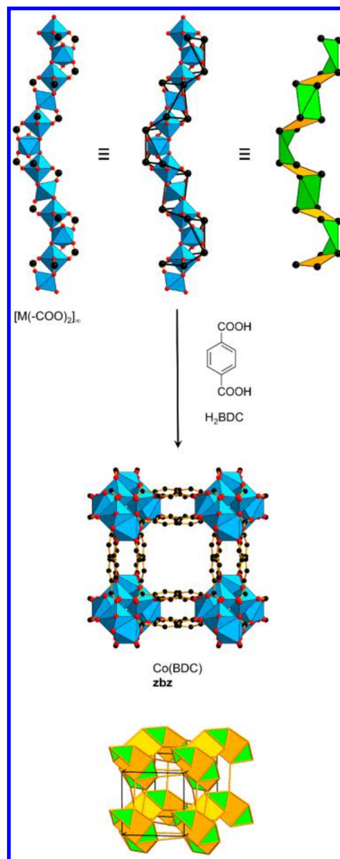
Figure 71. Crystal structure of \text{Co}(\text{BDC}) and the underlying (4,5)-c zbz net. The triangular and quadrangular SBUs form a 4-fold helix. 238 Color code: black, C; red, O; blue polyhedra, metal.
