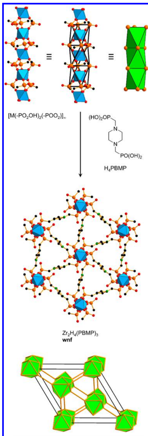
Figure 34. Crystal structure of Zr_2H_4(PBMP)_3 and its underlying uninodal 7-c net wnf . 169 Color code: black, C; red, O; green, N; orange, P; blue polyhedra, metal.
