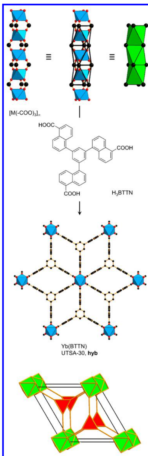
Figure 38. Linking of face-sharing octahedra with a triangular tricarboxylate produces UTSA-30, a framework with hyb topology. 29 Color code: black, C; red, O; blue polyhedra, metal.
