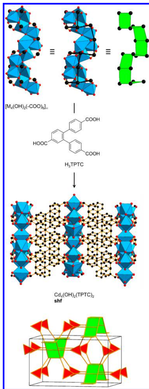
Figure 73. Crystal structure of \text{Cd}_4(\text{OH})_2(\text{TPTC})_2 built of double-crankshaft chains linked through tritopic linkers into an overall (3,4)-c shf net. 239 Color code: black, C; red, O; blue polyhedra, metal.
