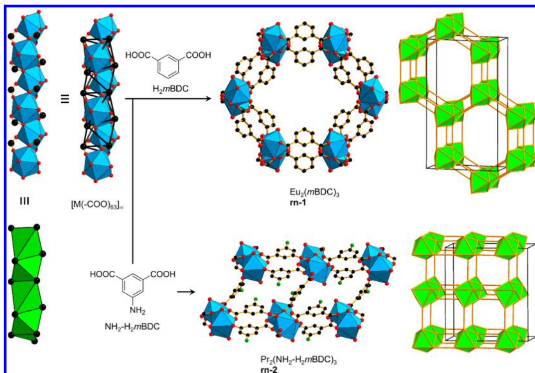
Figure 35. Linking of face-sharing octahedral SBU, [M(-\text{COO})_3]_\infty , with angular dicarboxylates leading to different nets. 171,172 Color code: black, C; red, O; green, N; blue polyhedra, metal.
