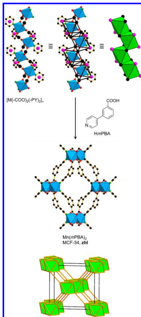
Figure 37. Combination of opposite and adjacent edge-sharing octahedral SBUs [M(-COO)_2(-PY)_2]_\infty and the underlying zh1 net. 173 Color code: black, C; red, O; green, N; blue polyhedra, metal; pink, points of extension.
