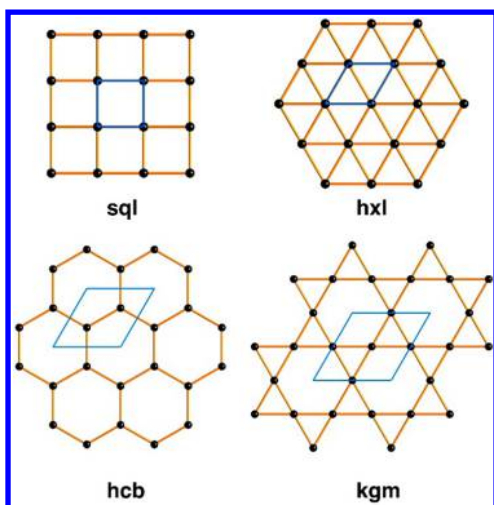
Figure 6. Invariant 2-periodic patterns.
