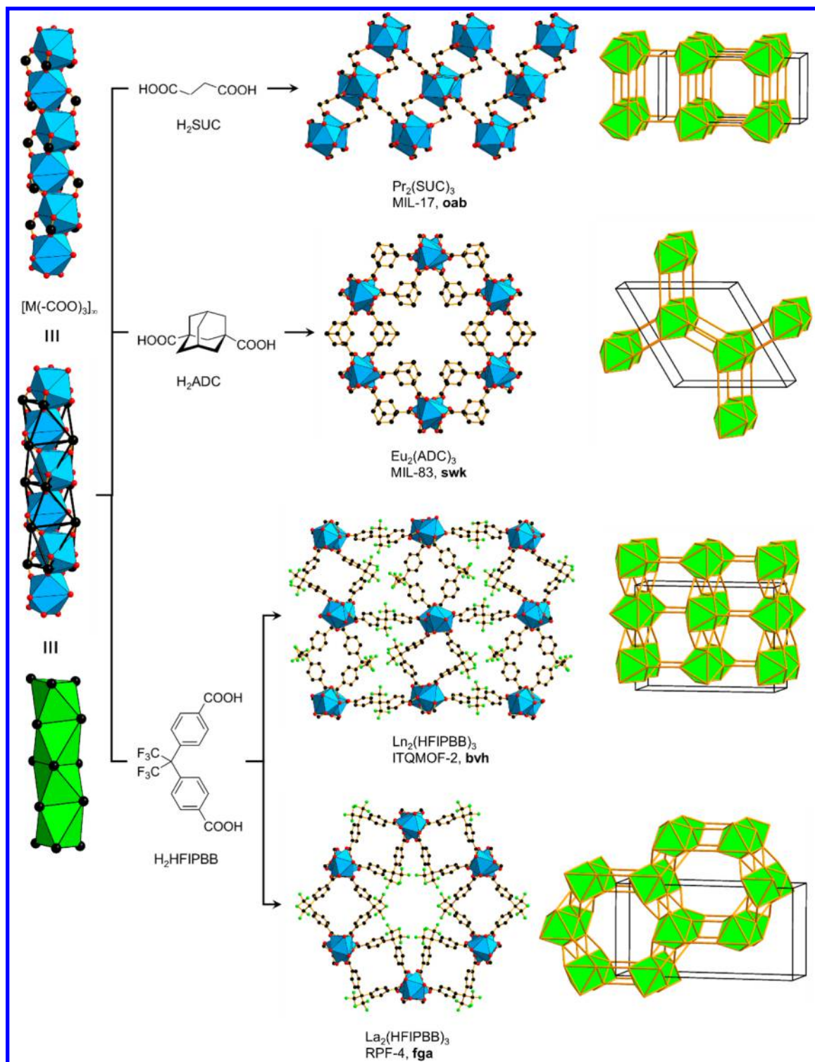
Figure 32. Linking of face-sharing octahedral SBUs, [M(-COO)_3]_{\infty} , with rigid and flexible dicarboxylates leads to a large structural diversity exemplified by oab , 155 swk , 160 bvh , 164 and fga nets, 165 respectively. Color code: black, C; red, O; green, F; blue polyhedra, metal.
