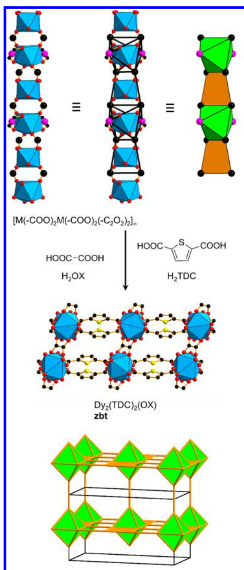
Figure 61. Crystal structure of \text{Dy}_2(\text{TDC})_2(\text{OX}) and the underlying zbt net. 228 Color code: black, C; red, O; blue polyhedra, metal; pink, points of extension.
