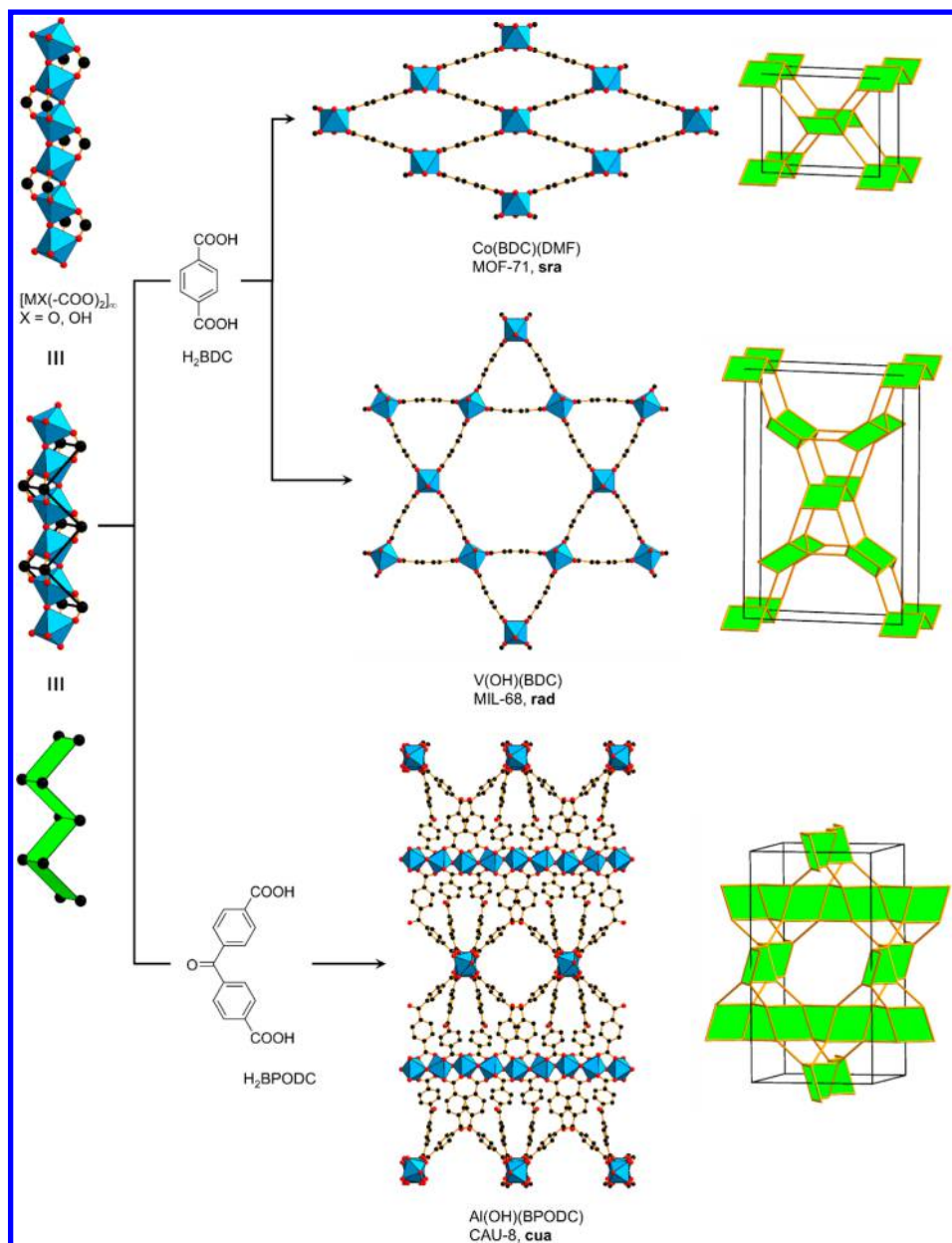
Figure 16. Three topologically different frameworks formed by zigzag ladders of general formula [MX(-COO)_2]_\infty ( X = O, OH ). Various angles subtended either at the SBU or the linkers facilitate different orientation of rod SBUs in 1-dimension ( sra , rad ) or in 2-dimensions ( cua ). 6,114,116 Color code: black, C; red, O; blue polyhedra, metal.
