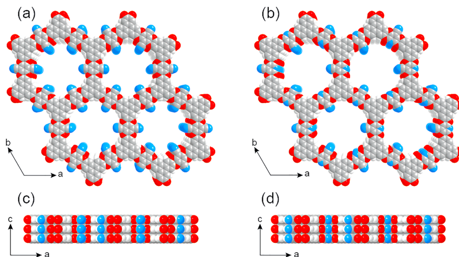
Figure 3. (a, b) Top views and (c, d) side views of the space-filling models of COF-316 and -318 in eclipsed stacking mode. Color code: H, white; C, gray; N, blue; O, red.
