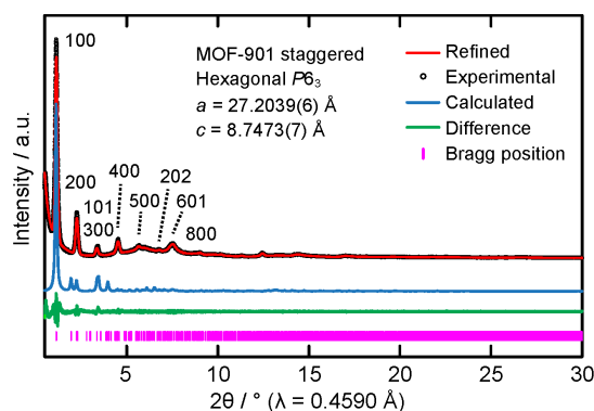
Figure 2. PXRD analysis of activated MOF-901 displaying the experimental pattern (black), refined Pawley fitting (red), and calculated pattern from the staggered structural model (blue). The difference plot (green) and Bragg positions (pink) are also provided.
