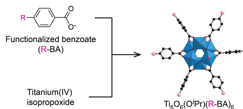
Scheme 1. Synthetic scheme depicting the generalized formation of a discrete hexameric titanium cluster, which can be appropriately functionalized with amine groups to affect imine condensation reactions. Atom colors: Ti, blue; C, black; O, red; R groups, pink; H atoms and capping isopropoxide units are omitted for clarity.
