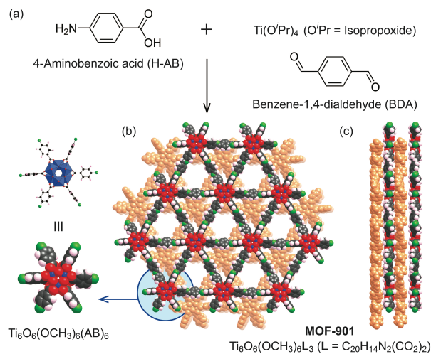
Figure 1. MOF-901 was synthesized by exploiting the robust conditions used to form the discrete hexameric Ti(IV) oxo cluster. In forming MOF-901, 4-aminobenzoic acid was judiciously chosen to generate in situ amine-functionalized hexameric clusters, which were, in turn, stitched together through imine-condensation reactions involving benzene-1,4-dialdehyde (a). The crystal structure of MOF-901 is projected along c -axis (b) and a -axis (c). The discrete hexameric cluster, now incorporated into an extended, crystalline structure, is presented in the inset of (b). Atom colors: Ti, blue; C, black; O, red; N, green; H, pink; and second layer, orange. Capping methoxide moieties are removed for clarity.
